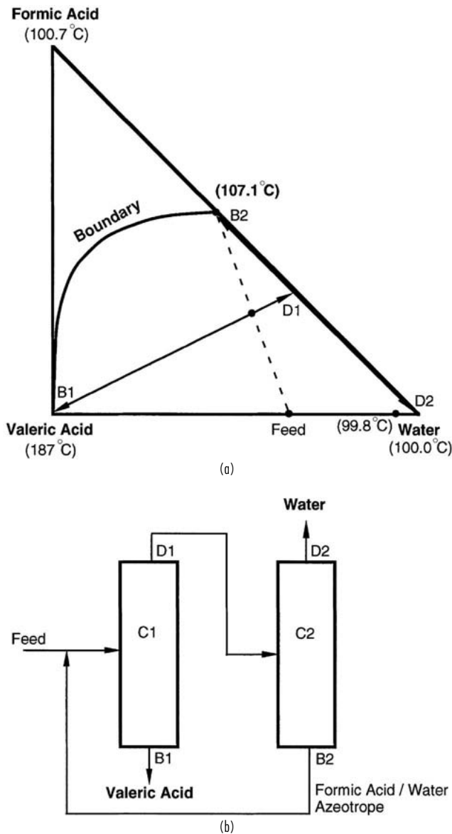
FIG. 13-85 Valeric acid-water separation with formic acid. (a) Mass balances on distillation region diagram. (b) Conceptual sequence.
