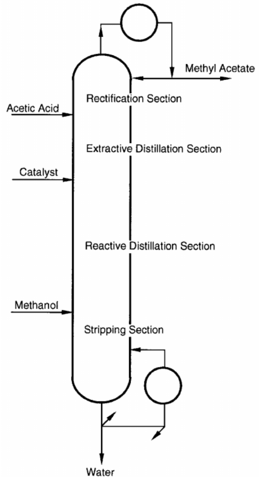
FIG. 13-99 Integrated reactive-extractive distillation column for the production of methyl acetate.
