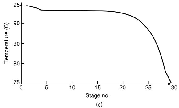
FIG. 13-82 Sensitivity of composition and temperature profiles for MEK-MIPK-water system at 1 atm.
