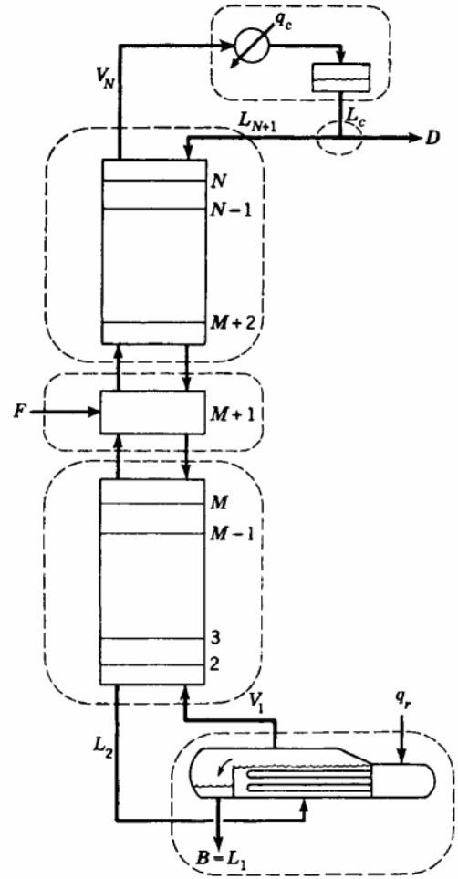
FIG. 13-62 Distillation column with one feed, a total condenser, and a partial reboiler.
