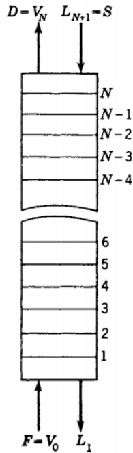
FIG. 13-61 Simple absorption column.
