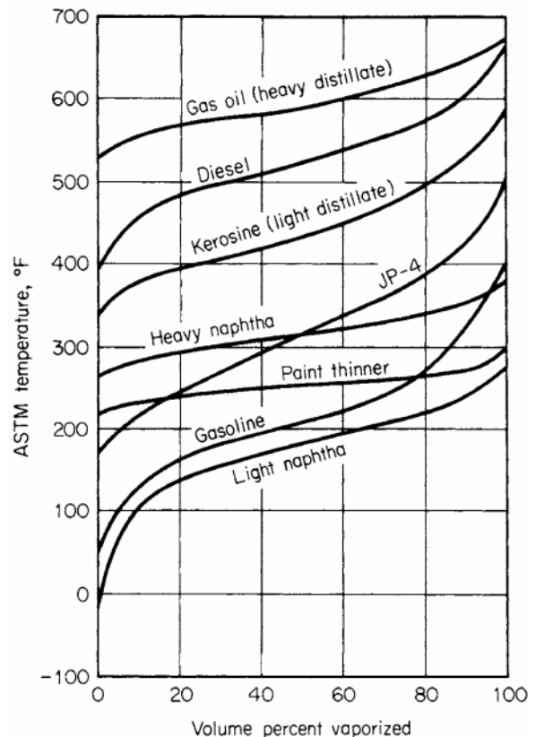
FIG. 13-102 Representative ASTM D 86 distillation curves.
