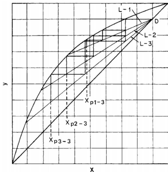
FIG. 13-125 Schematic of constant distillate composition operation.
