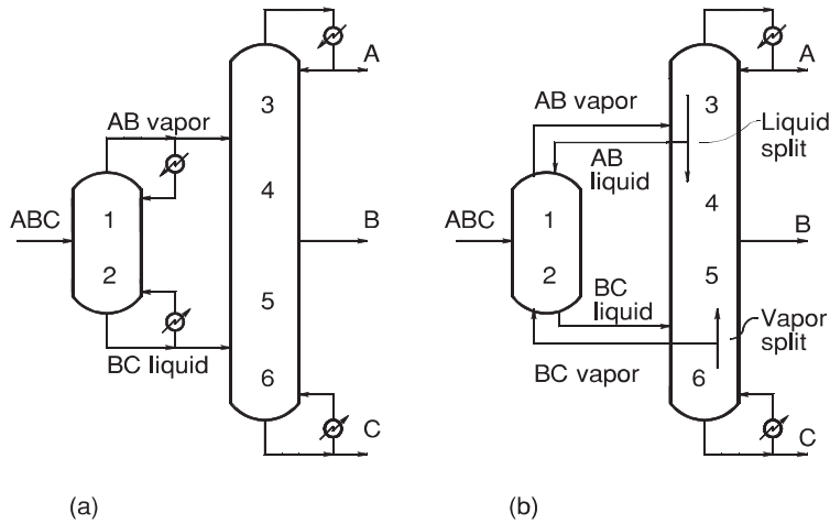
FIG. 13-67 (a) Prefractionator system. (b) Thermally coupled system.
