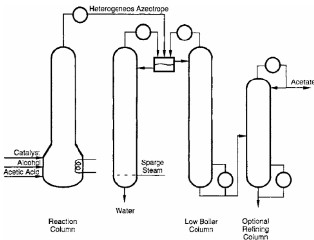
FIG. 13-98 Flow sheet for making esters which form a heterogeneous minimum-boiling azeotrope with water.
