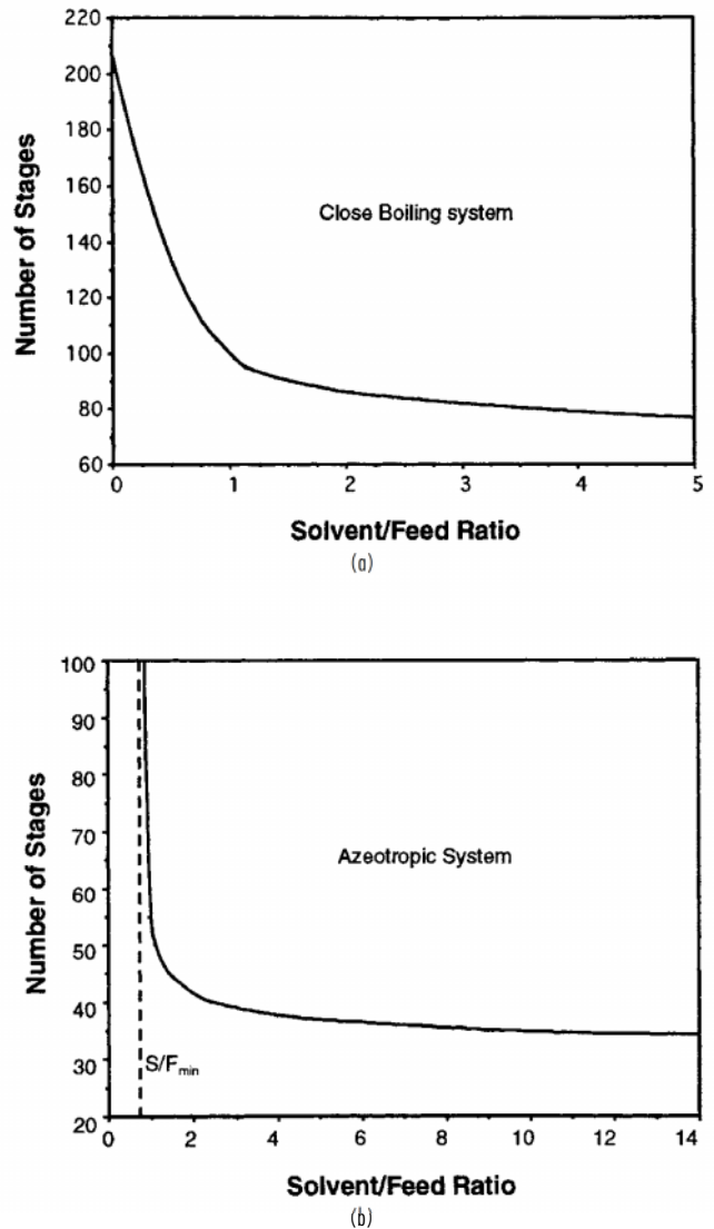
FIG. 13-95 Number of theoretical stages versus solvent-to-feed ratio for extractive distillation. (a) Close-boiling vinyl acetate-ethyl acetate system with phenol solvent. (b) Azeotropic acetone-methanol system with water solvent.
