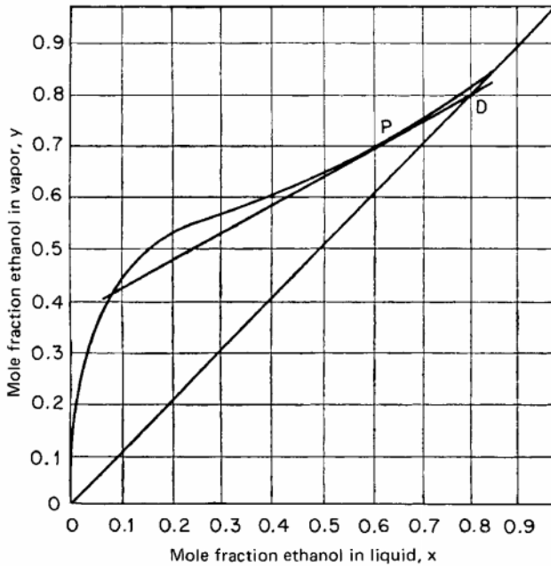
FIG. 13-123 Determination of minimum reflux for an equilibrium curve with an inflection point.
