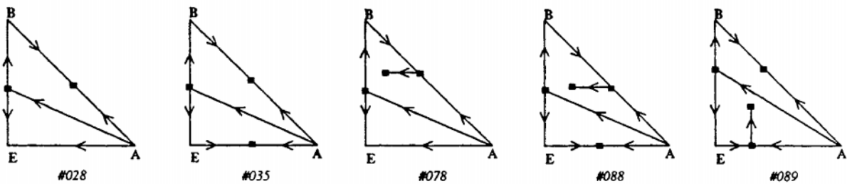
HIGH-BOILING ENTRAINER.
