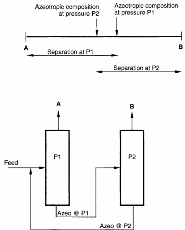
FIG. 13-86 Conceptual sequence for separating maximum-boiling binary azeotrope with pressure-swing distillation.
