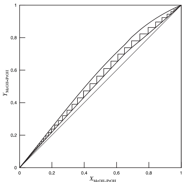
FIG. 13-57 McCabe-Thiele diagram for nonideal distillation column.
