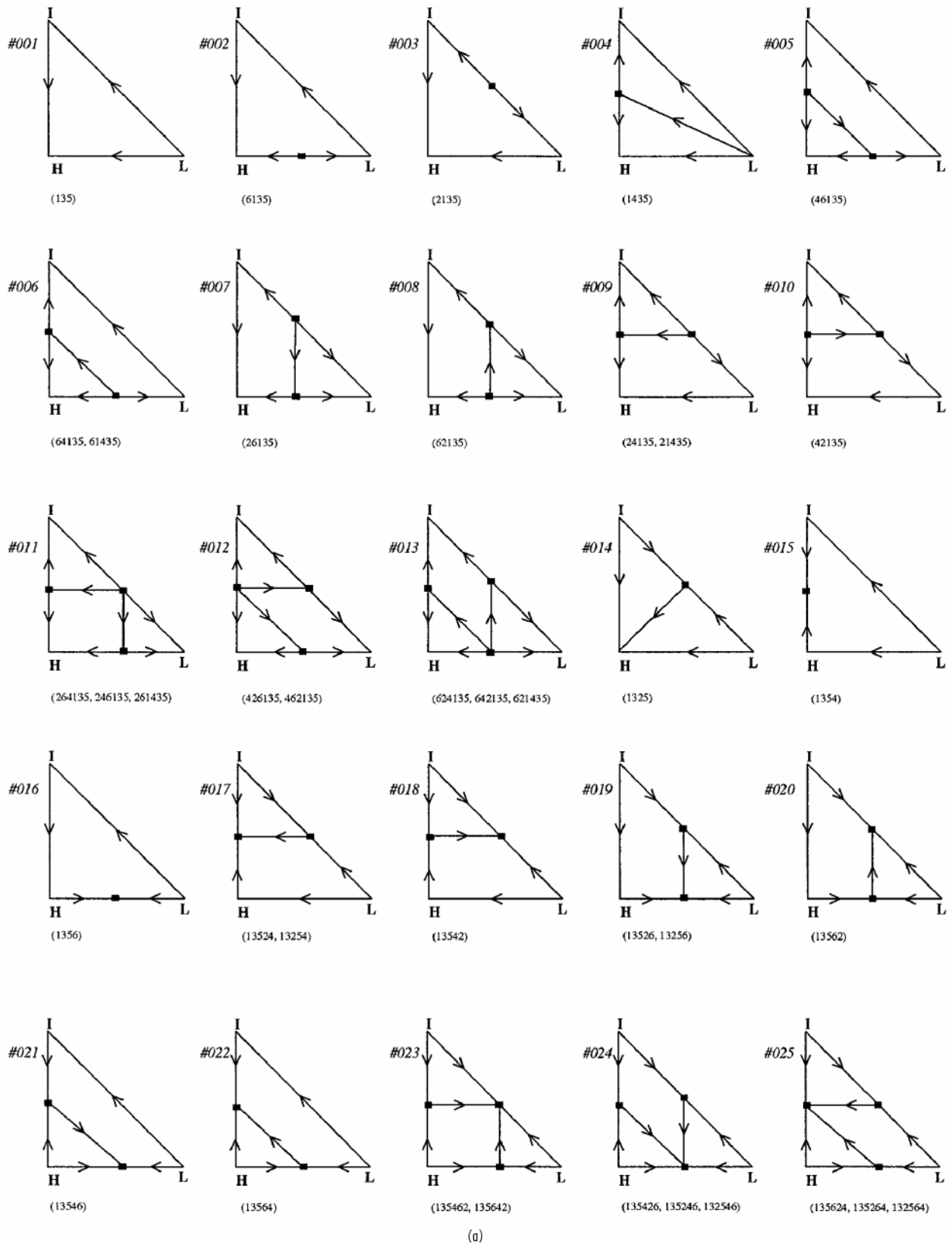
FIG. 13-79 Distillation region diagrams for ternary mixtures.
