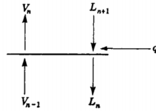
FIG. 13-60 Simple equilibrium stage.
