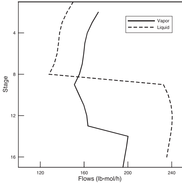
FIG. 13-45 Flow profiles in hydrocarbon distillation in Fig. 13-43.
