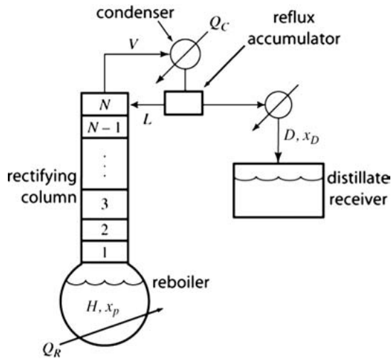
FIG. 13-119 Schematic of a batch rectifier.
