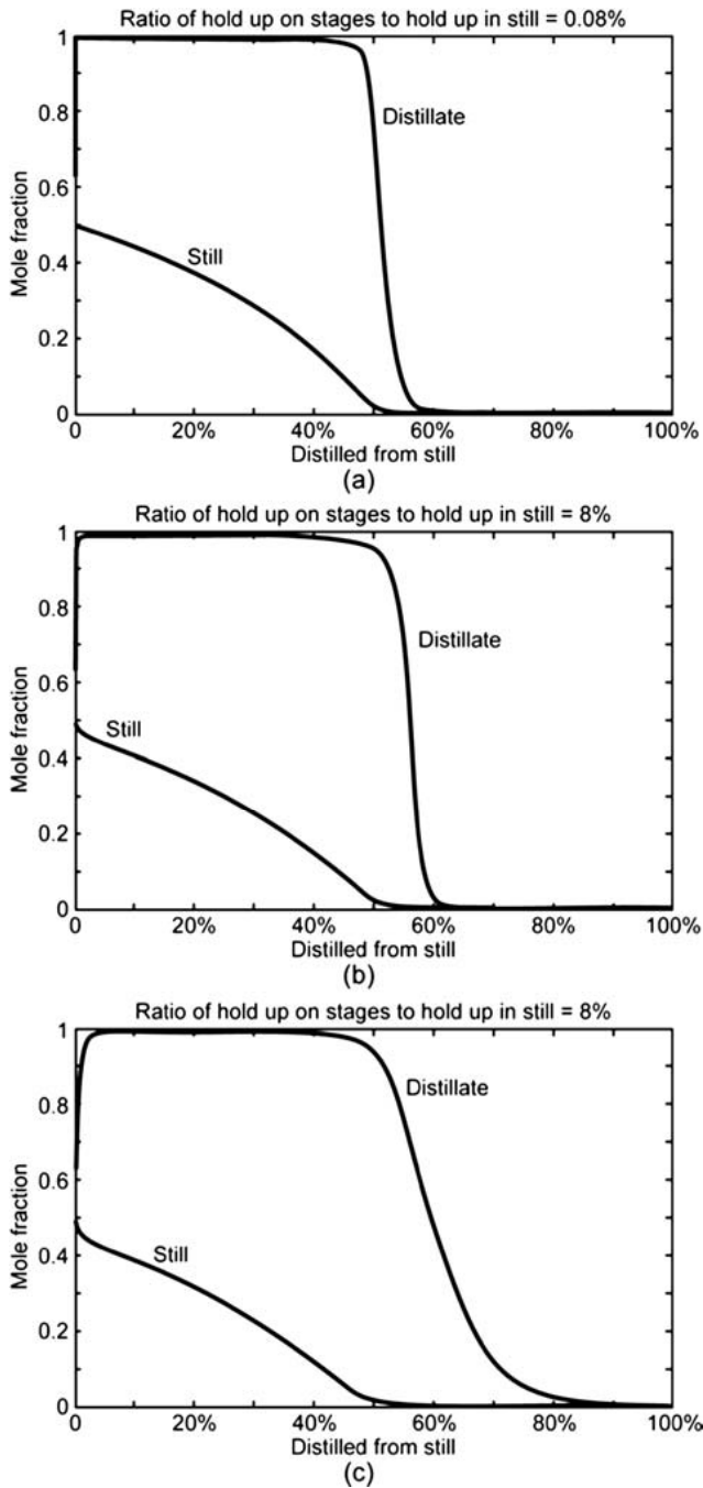
FIG. 13-127 Effects of holdup on batch rectifier.
