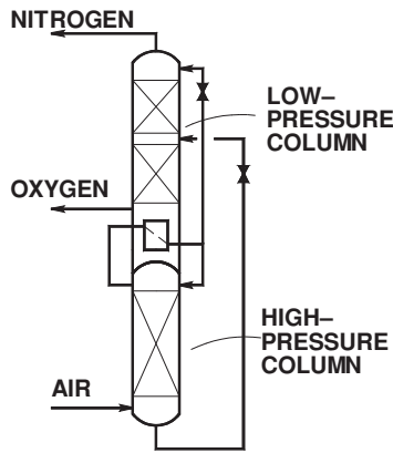
FIG. 13-76 Double-column arrangement for air separation.
