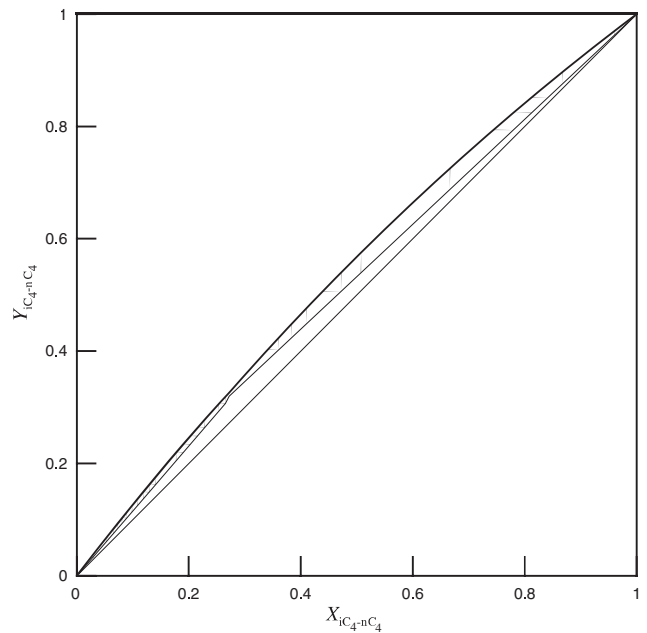
FIG. 13-50 McCabe-Thiele diagram for C_4 splitter.
