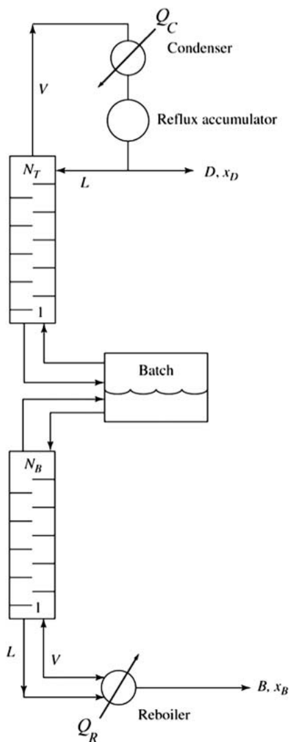
FIG. 13-129 Middle vessel batch distillation.
