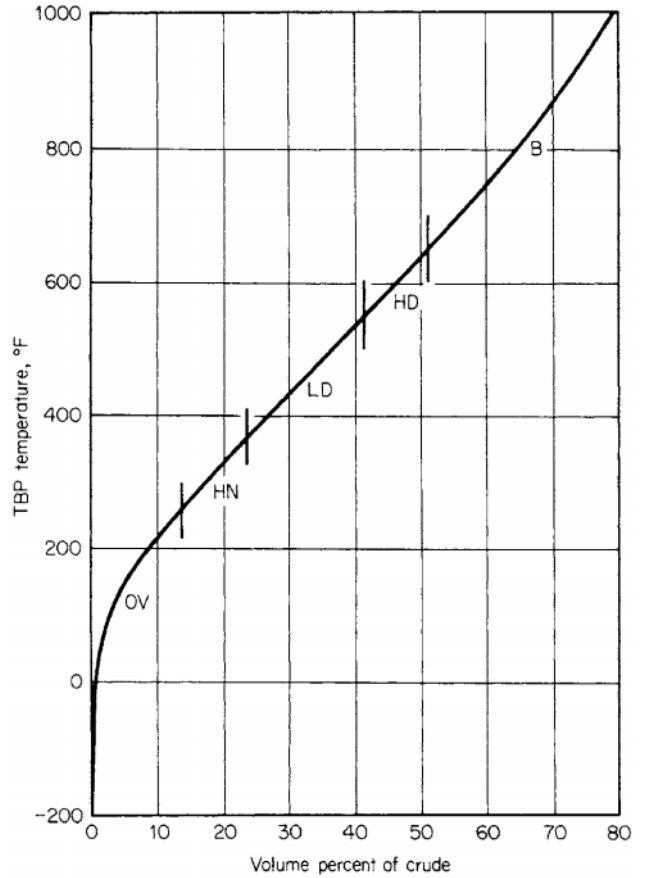
FIG. 13-111 Example of crude oil TBP cut points.
