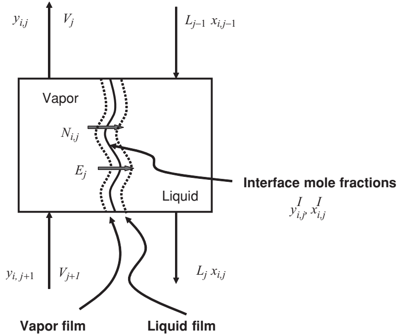
FIG. 13-54 Schematic diagram of a nonequilibrium stage.
