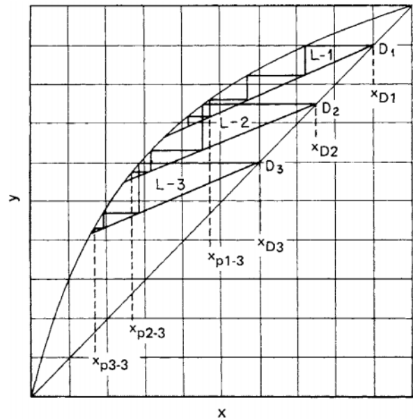
FIG. 13-124 Graphical method for constant-reflux operation.
