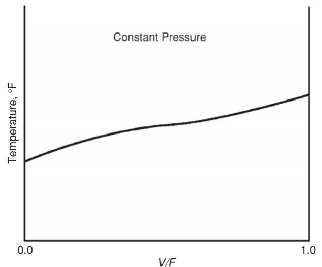
FIG. 13-17 Equilibrium flash curve.
